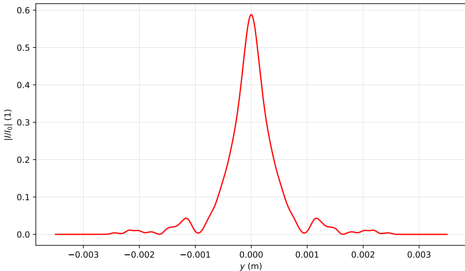
Intensity profile I(x = 0, y, z = 2.388)/I_0 , P_{in}=4.5P_{cr} , artificial time
